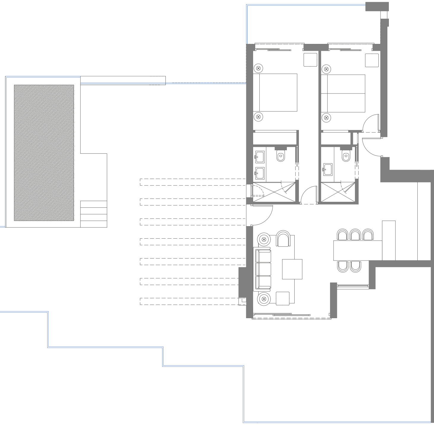
APARTMENT 121 (LEVEL 104)
