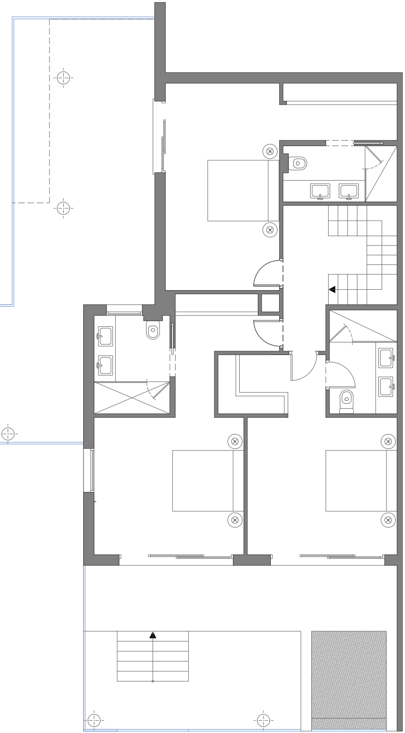
GROUND FLOOR DUPLEX 101
